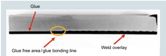
Fig. 2: Pipe end configuration incl. glue free area (metallographic cross section)
