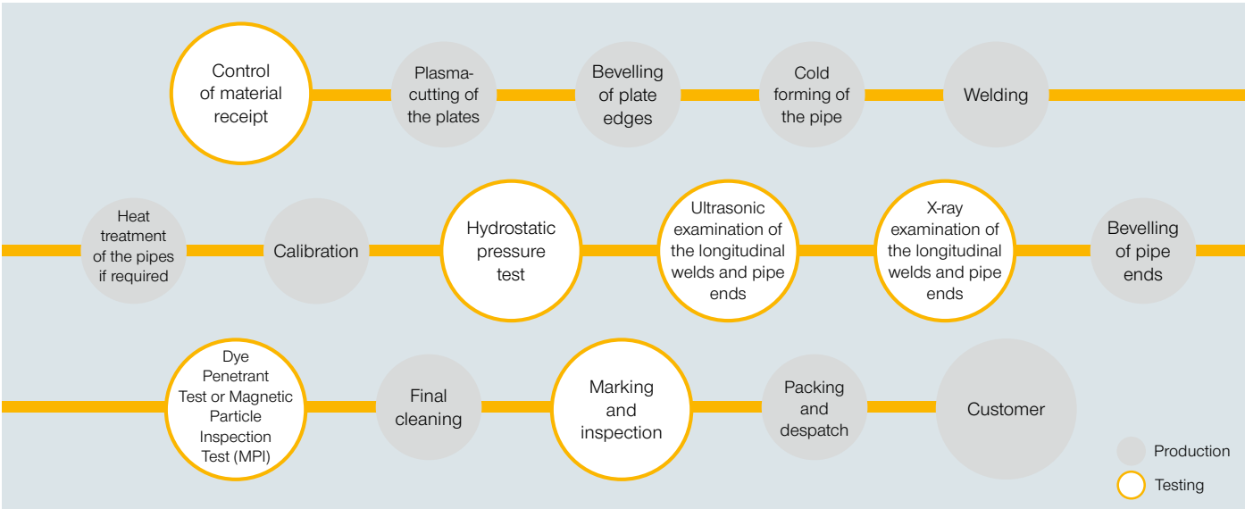
Manufacturing route of metallurgically clad pipes
